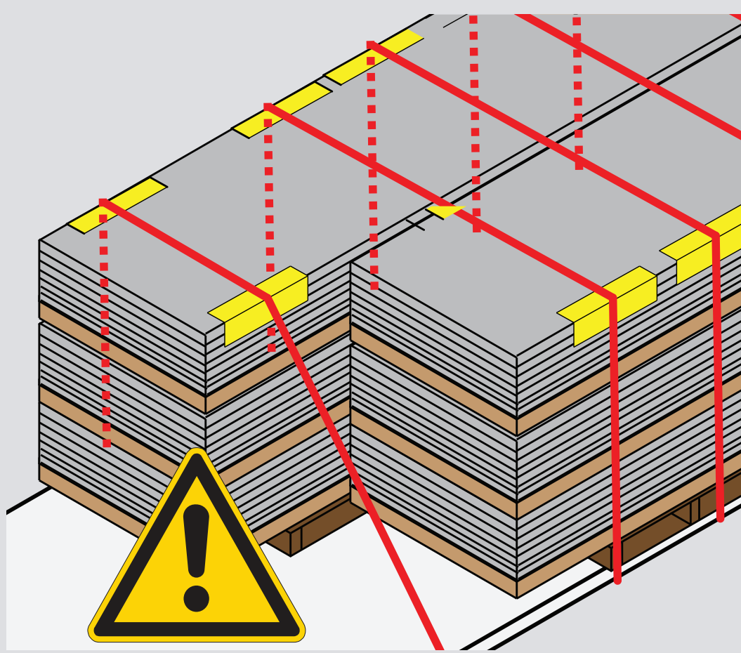
Lashings applied over part of the load do not count towards total lashing requirements in tables
