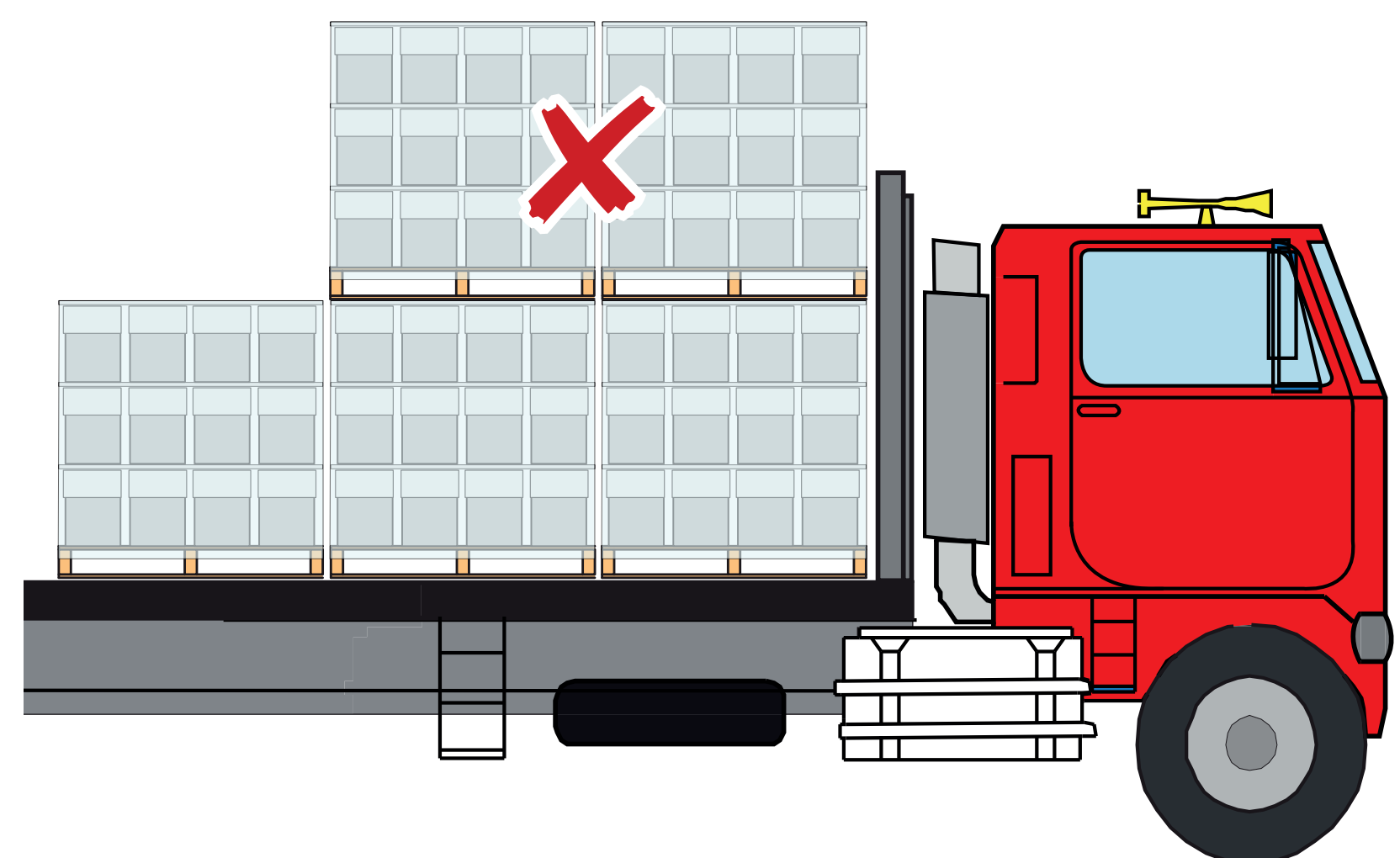
Do not exceed height of headboard The maximum height of a vehicle including any load that is placed on it (measured from the ground) must not exceed 4.3 metres
