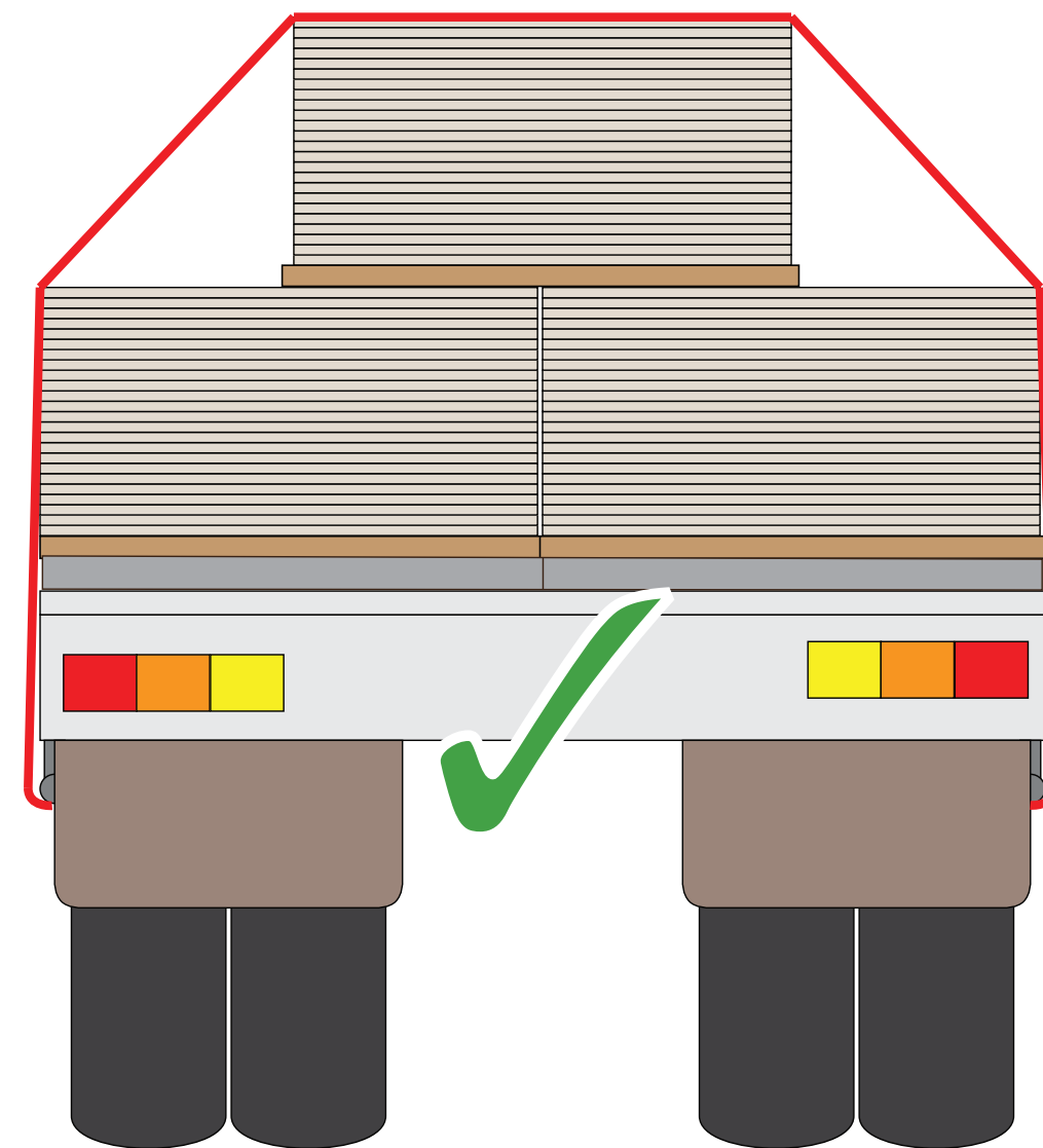
Pyramid stack loads of 3 bundles
